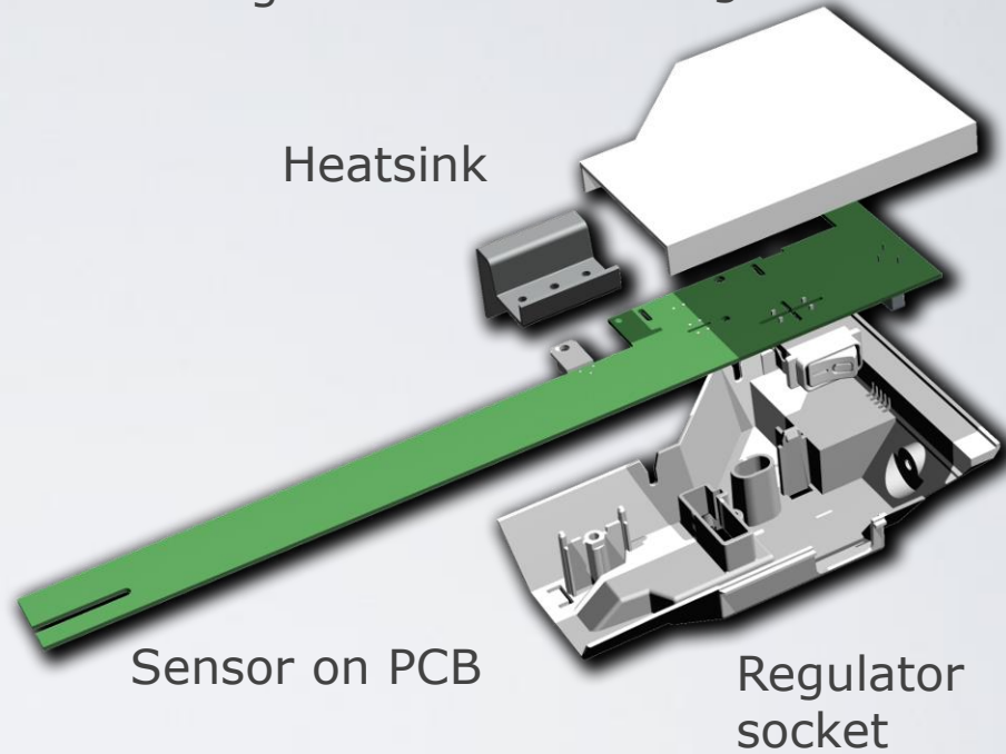
Regulator cover
