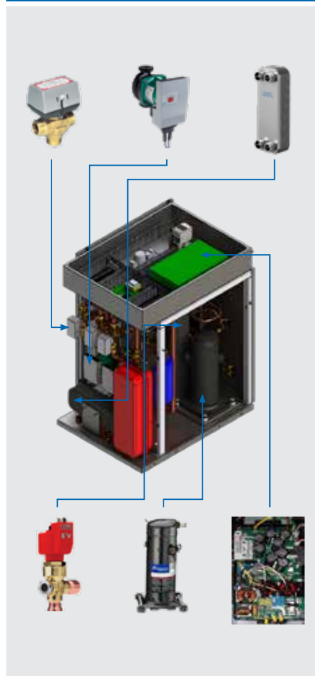
Vista interior
